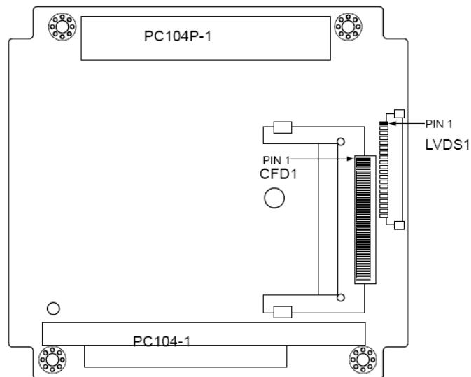
Figure 3: Pegasus Board Layout (bottom)
