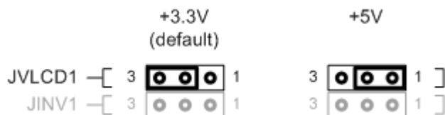
Figure 7: LVDS Panel Voltage Configuration
